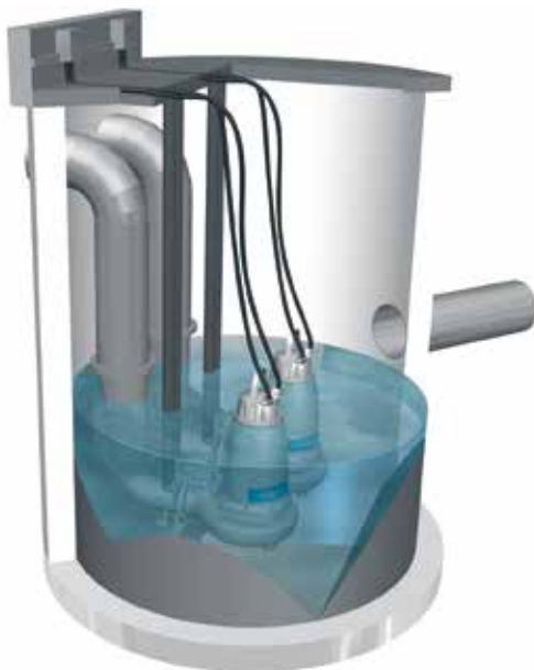
Non-submerged inlet.
