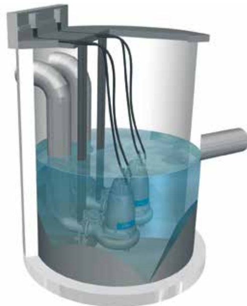
Submerged inlet.
