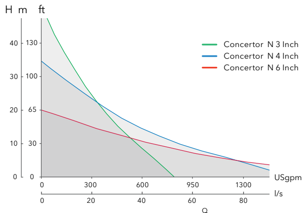
10HP / 380-480V / 3 phase
