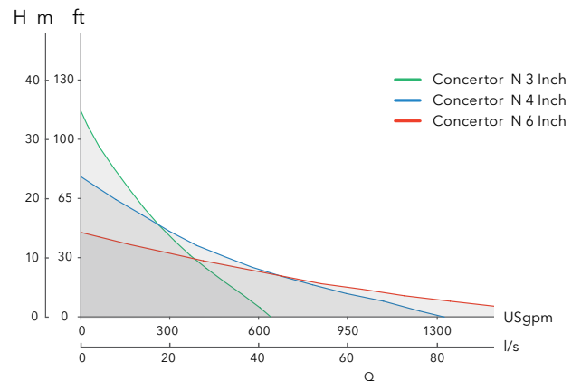
5.5HP / 200-240V / 3 phase
