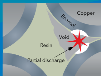
A partial discharge can destroy all organic parts of the insulation and lead to premature stator breakdown.
