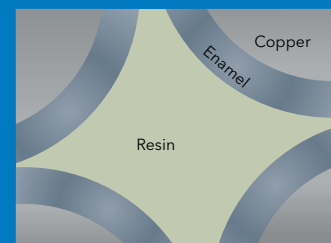
The impregnation techniques used in Flygt stators generate a solid resin fill.
